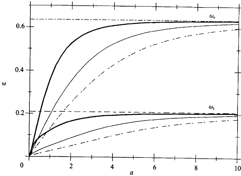
FIGURE 9. As figure 3, but for U = -1 , \alpha_0 = -0 , \alpha_s = -2 .
